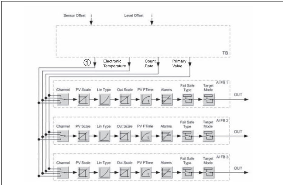
Рис. 26: MINITRAC 31: Block diagram with AI FB 1 ... AI FB 3 OUT values
