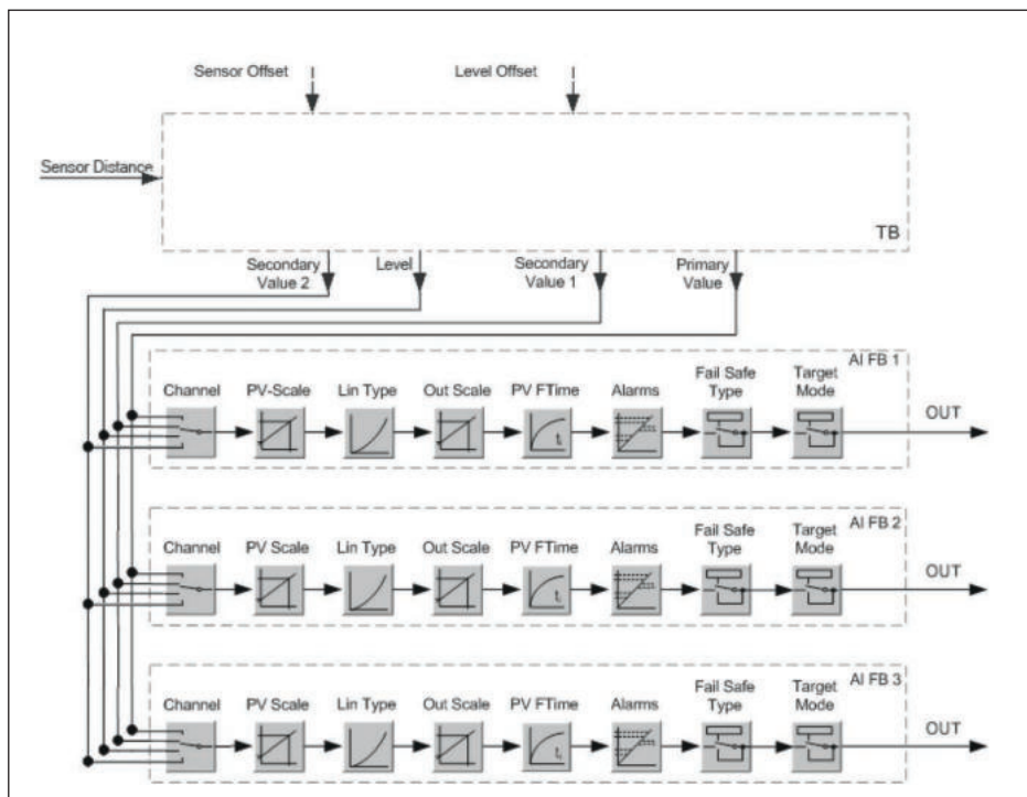
Рис. 38: VEGAFLEX 81: Block diagram with AI FB 1 ... AI FB 3 OUT values
