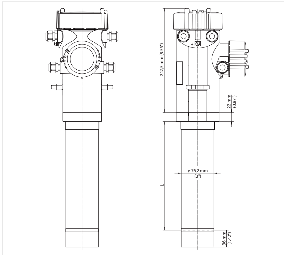
Рис. 29: SOLITRAC 31
