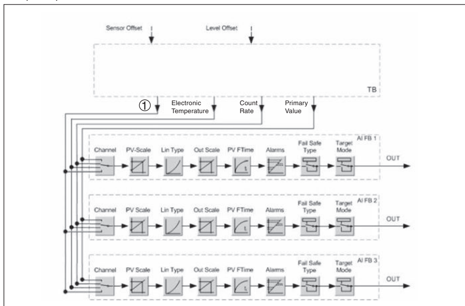
Рис. 25: SOLITRAC 31: Block diagram with AI FB 1 ... AI FB 3 OUT values
